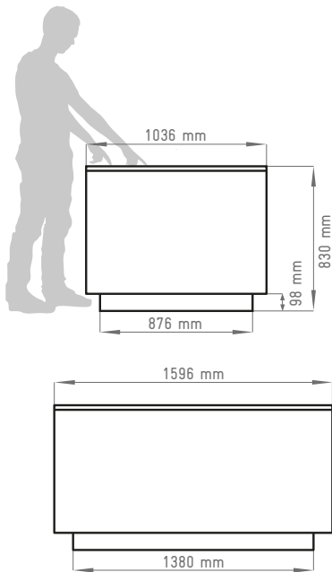
Transport case for the Struktable
